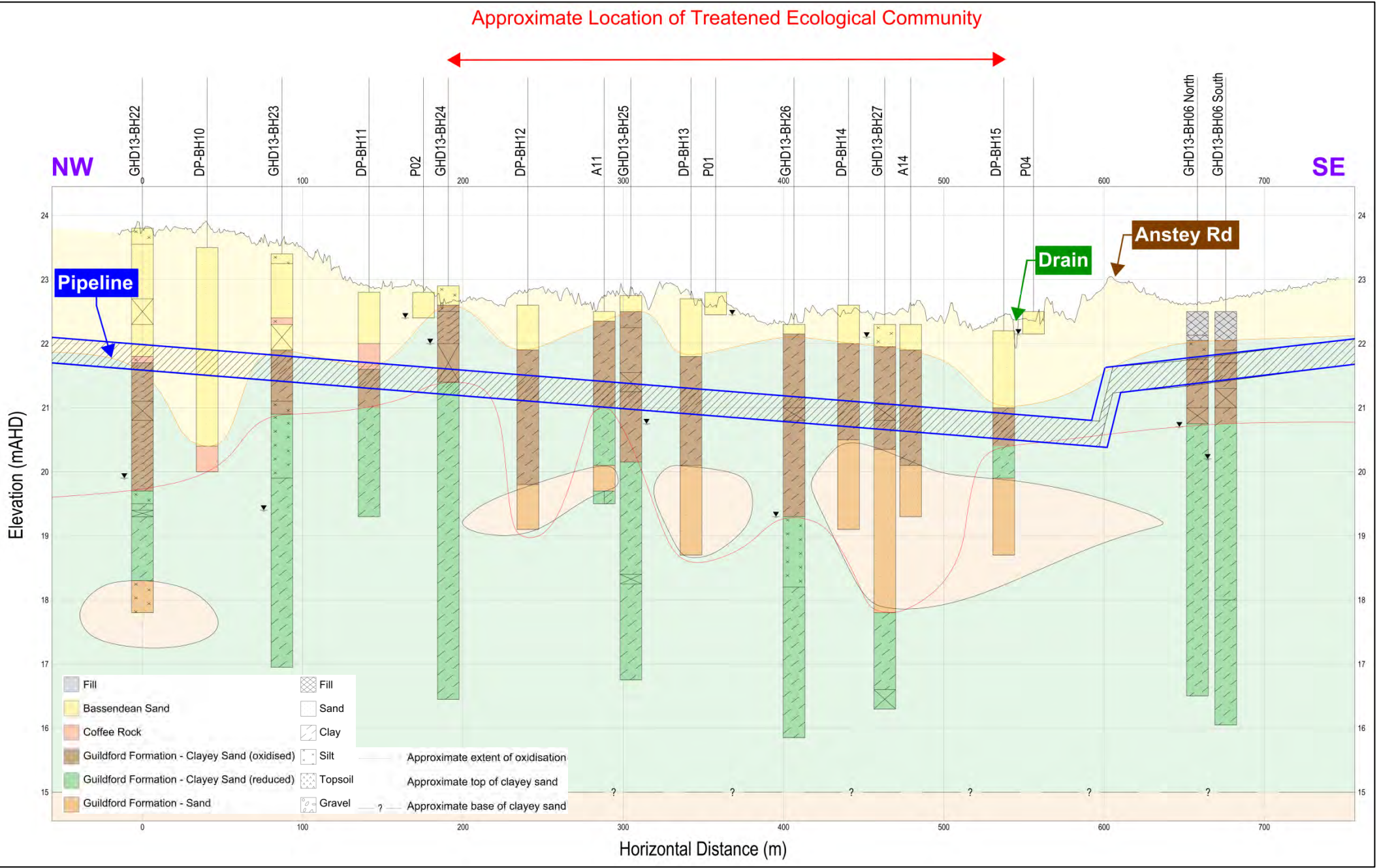
Figure 21: Section A along sewer main alignment
