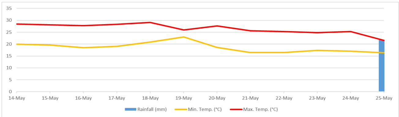
Figure 2.3: Daily Rainfall During the Phase 1 Survey (Fortescue’s Weather Station – North Star)
