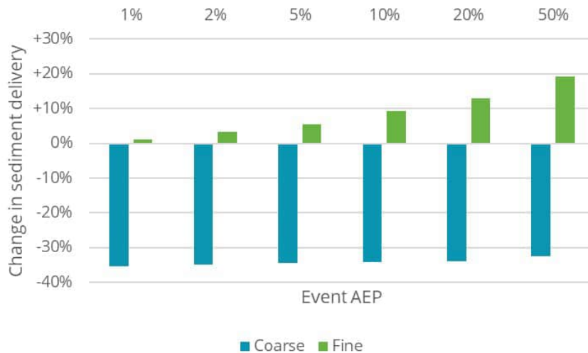
Figure 4-5: Changes in fine and coarse sediment delivery to Pool NJA19-002.
