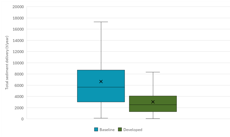
Figure 4-1: Box plots showing distribution of total sediment delivery for baseline and developed scenarios in Mundagoora Pool.
