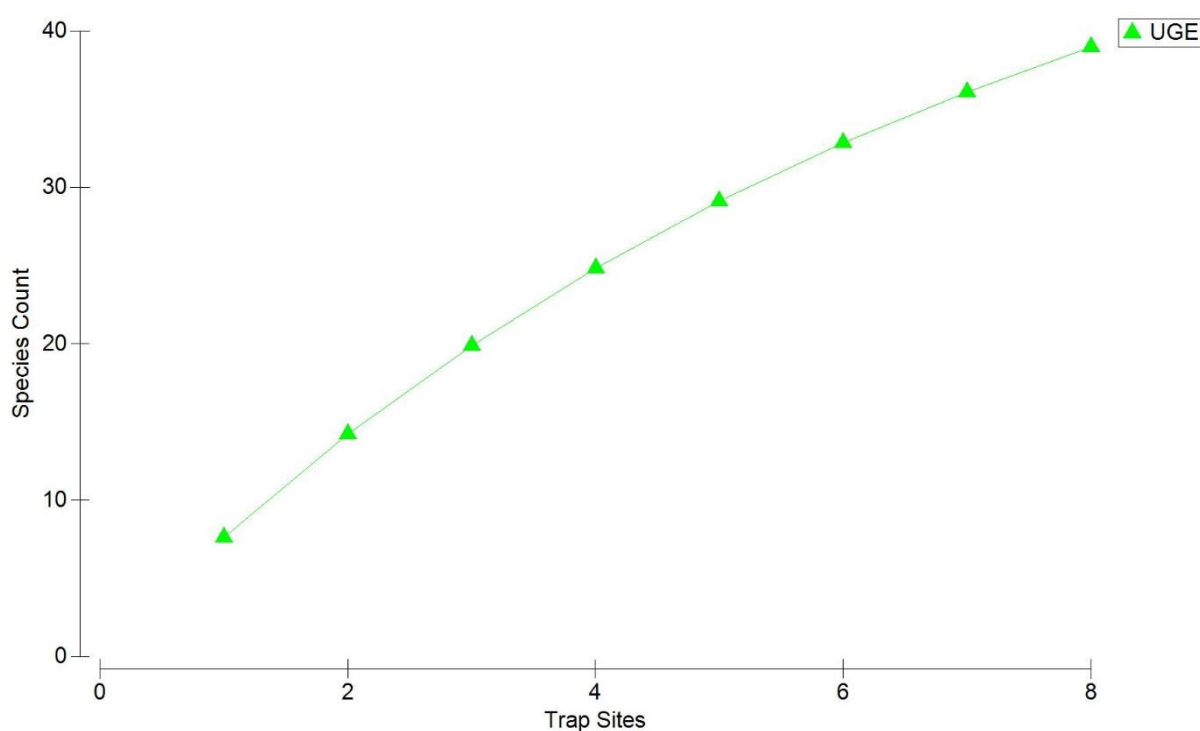
Chart 2 Accumulation curve of trap data combined
