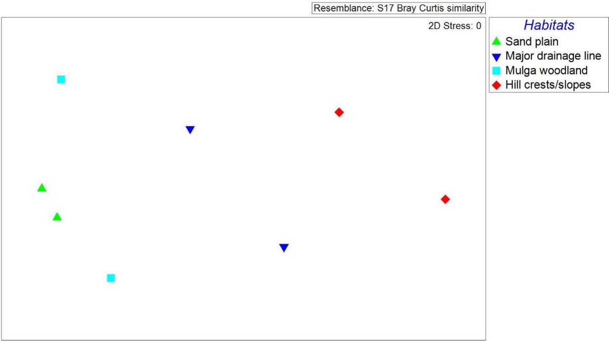
Chart 1 MDS of habitats based on species
