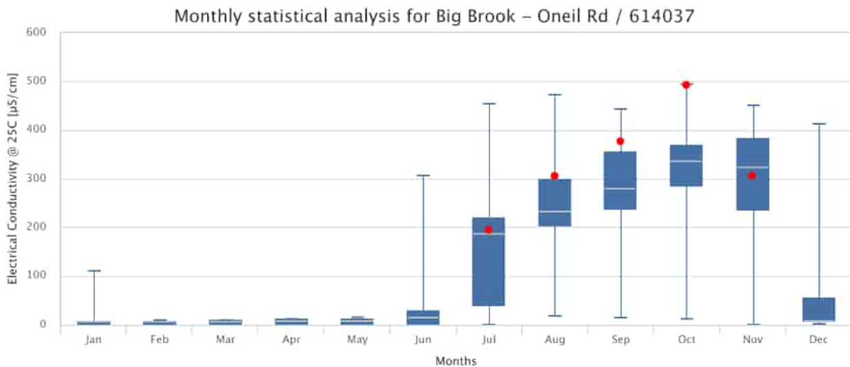
Figure 3.10 Long-term salinity trend at Big Brook (614037) over the monthly average salinity for 2022 (red dot)
