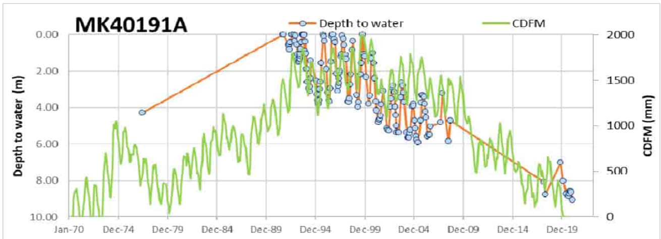
Figure 3.17 Long-term groundwater level trends at bore MK40191A (located within Myara North, north of Huntly DE) compared with cumulative deviation from mean monthly rainfall
