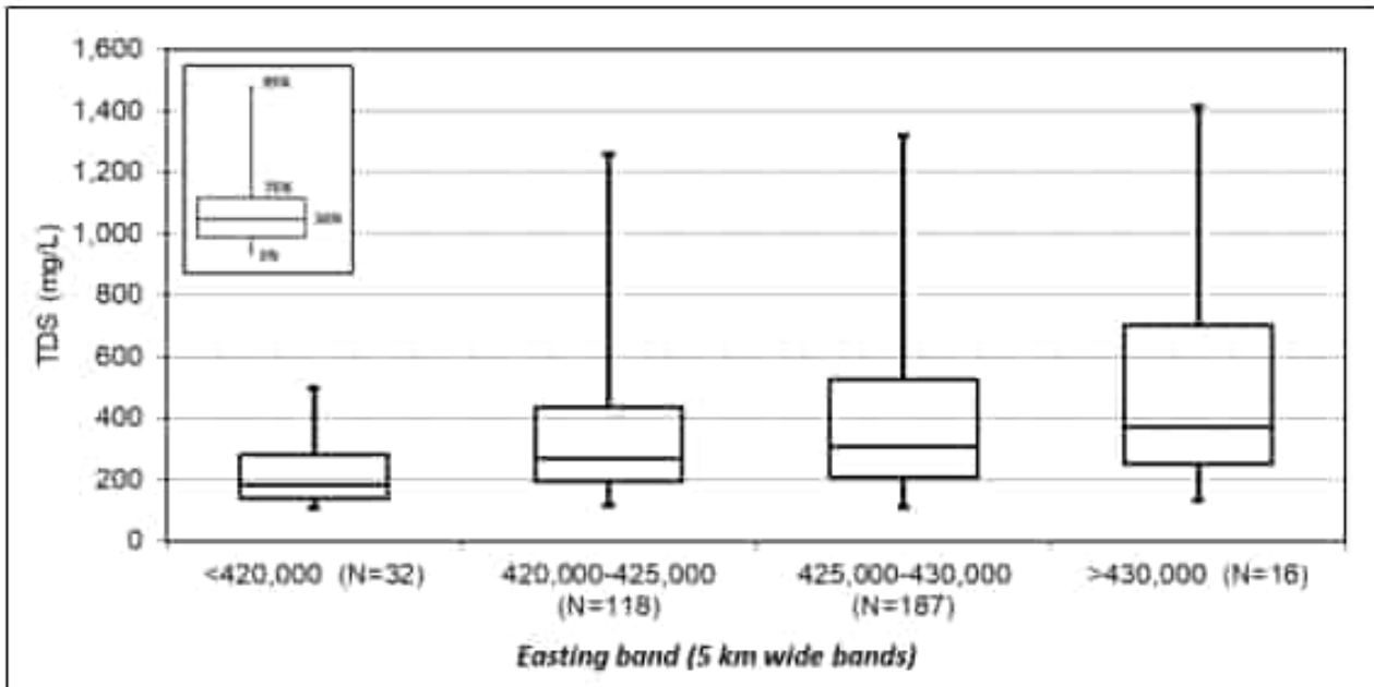
Figure 3.24 Groundwater salinity box and whisker plot (grouped by bore's Easting) (at Myara North, adjacent to Huntly DE) [after GHD (2021)]
