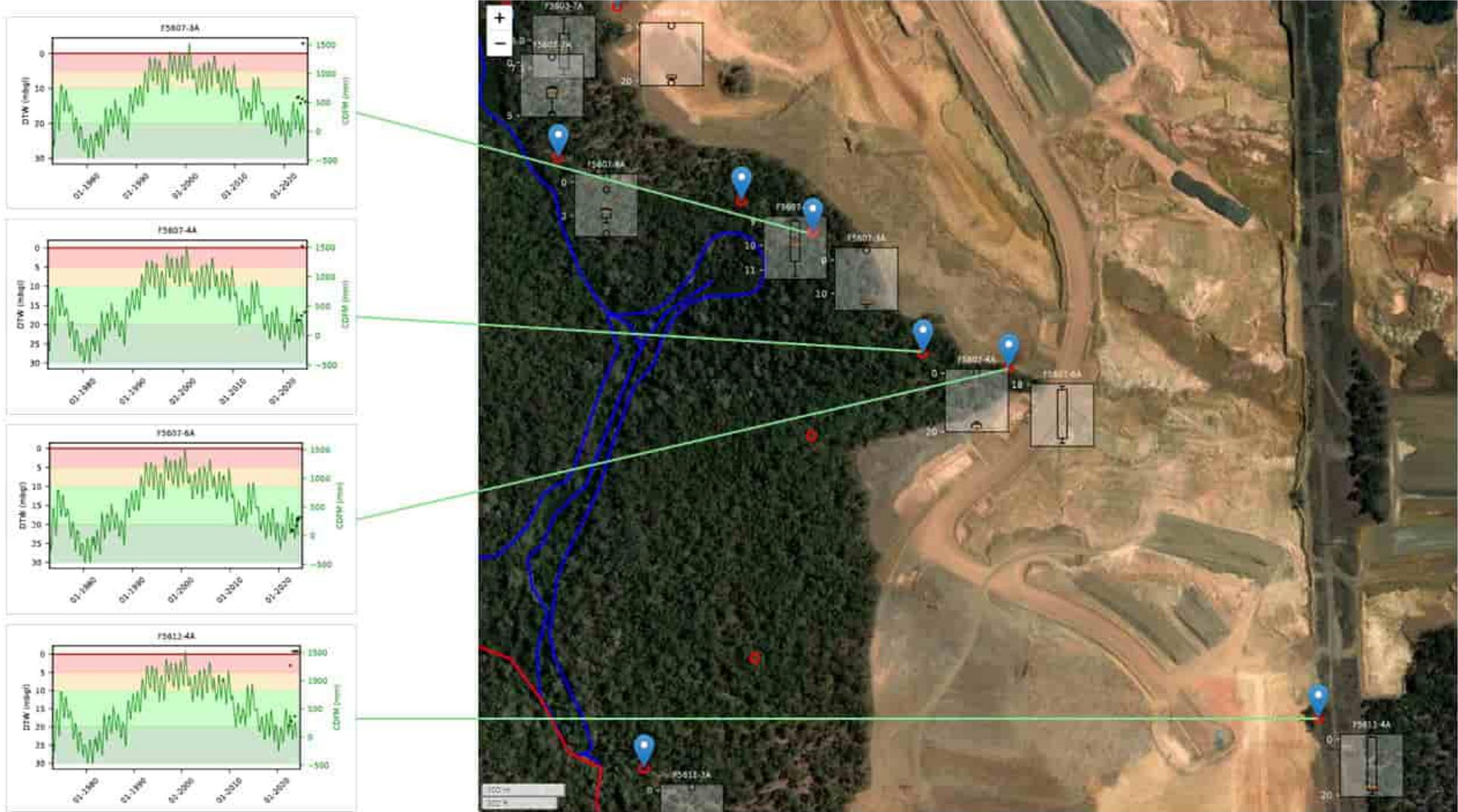
Figure 3.22 Groundwater level trends (bores F5607-3A, F5607-4A, F5607-6A, F5612-4A) within Larego mine region (Willowdale DE) in a mined portion of catchment compared with cumulative deviation from mean monthly rainfall
