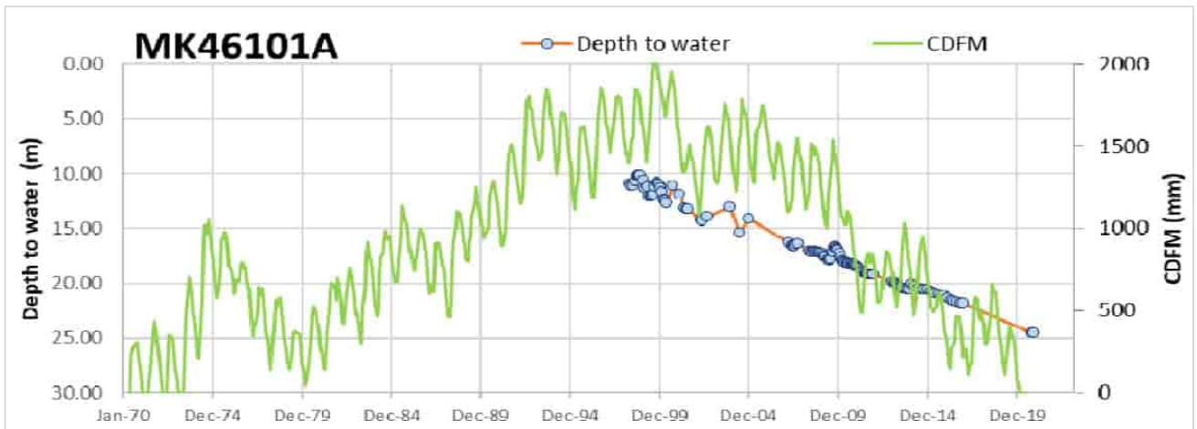
Figure 3.18 Long-term groundwater level trends at bore MK46101A (located within Holyoake, north of Willowdale DE) compared with cumulative deviation from mean monthly rainfall
