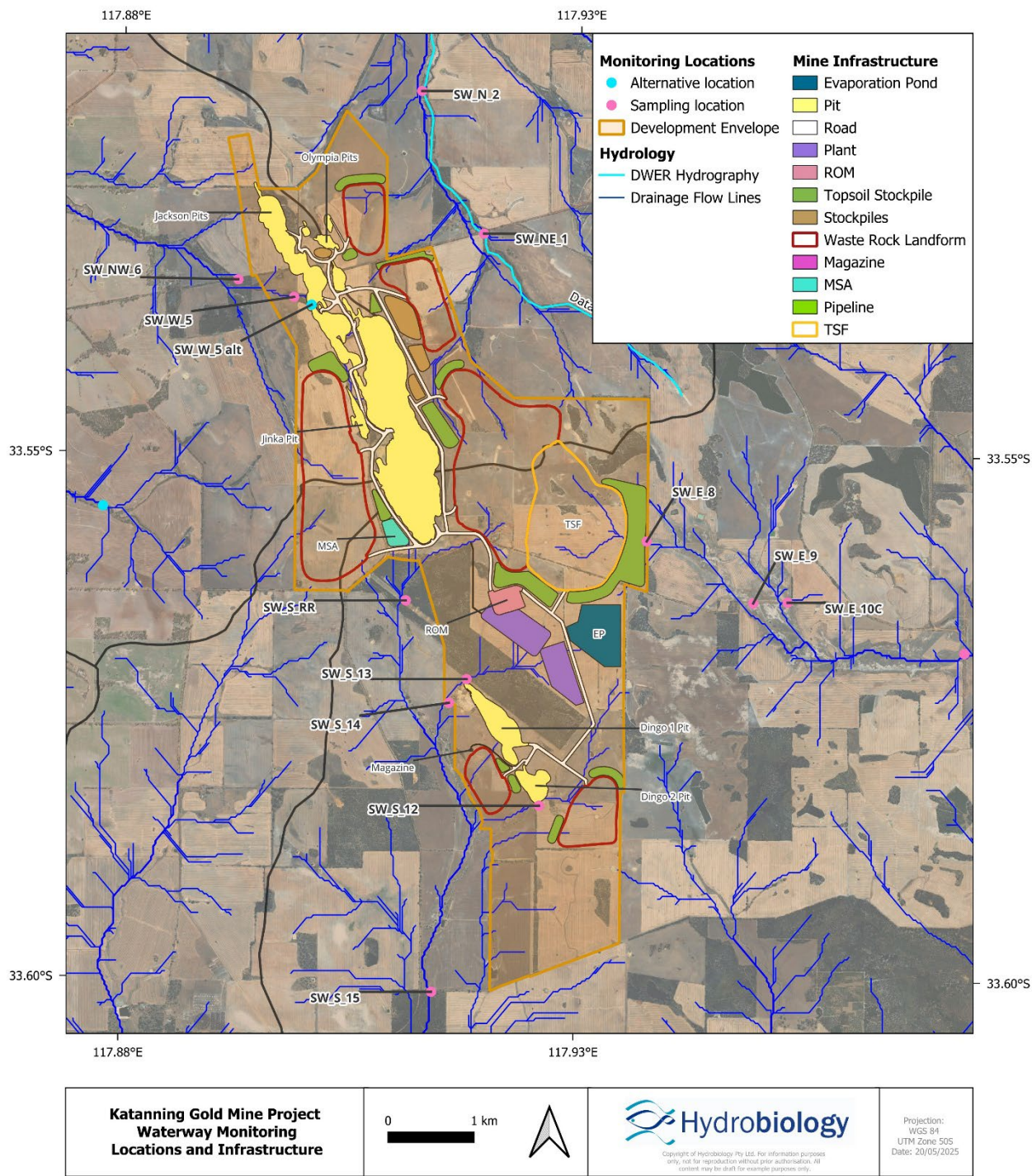
Figure 3 Proposed Mine Layout (Closeup)
