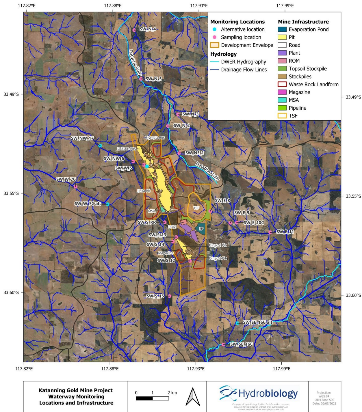
Figure 2 Proposed Mine Layout
