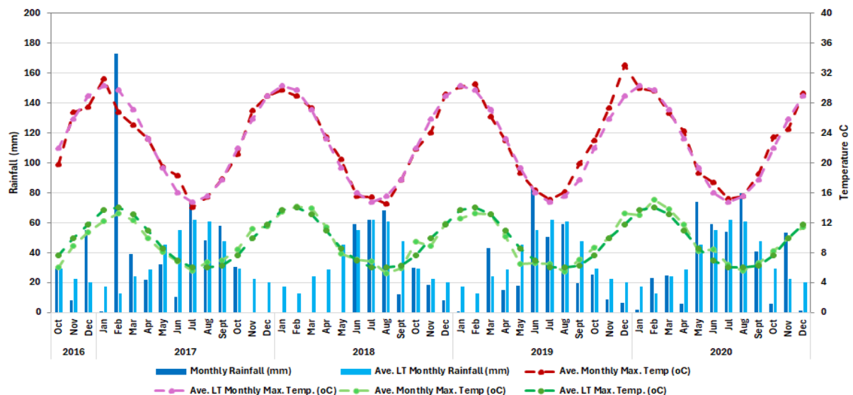
Figure 3.1: Rainfall and temperature data for Katanning recording station (2016 to 2020)
