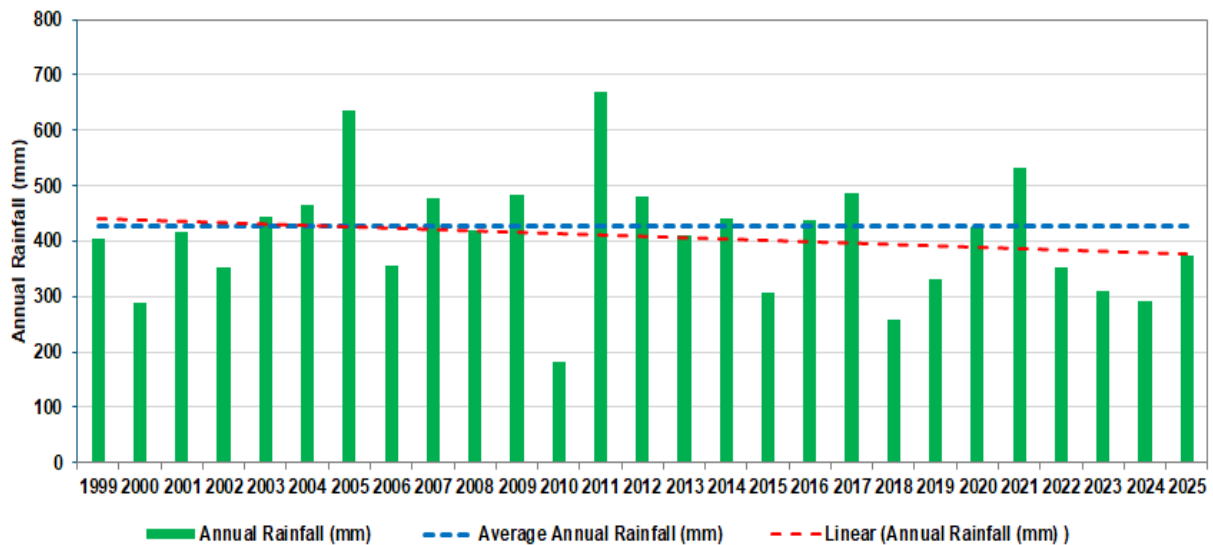
Figure 3.3: Longer Term Trends (showing Linear Trendline) for Rainfall from Katanning recording station (1999 to 2025)
