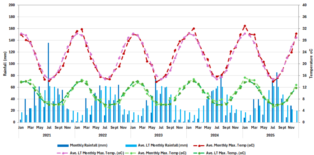
Figure 3.2: Rainfall and temperature data for Katanning recording station (2021 to 2025)
