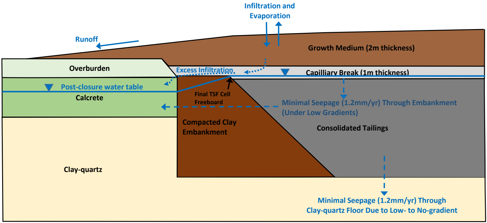
Figure 2: TSF Seepage Concepts
