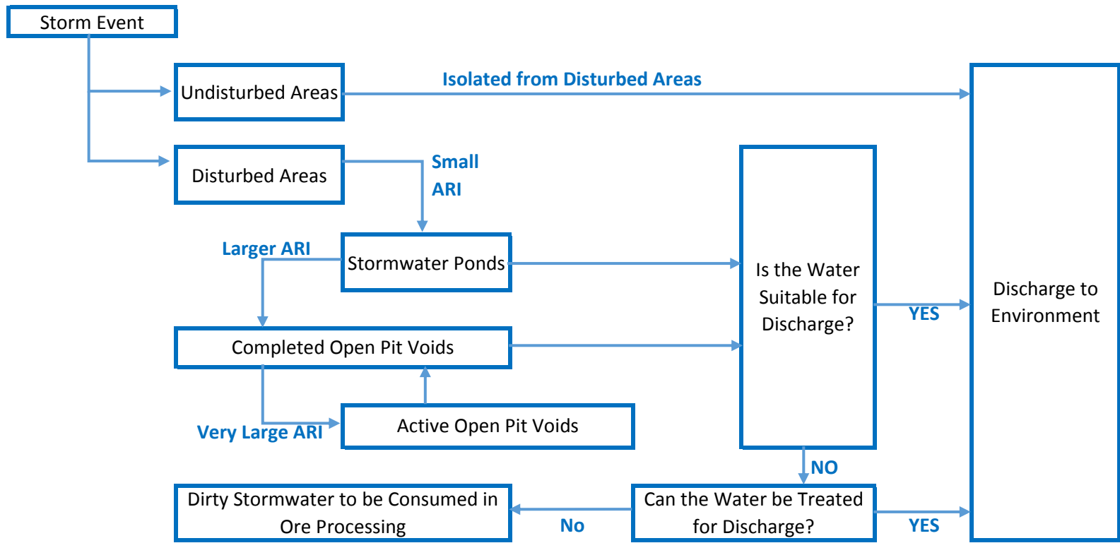
Figure 1: Stormwater Management and Environmental Discharge Concept
