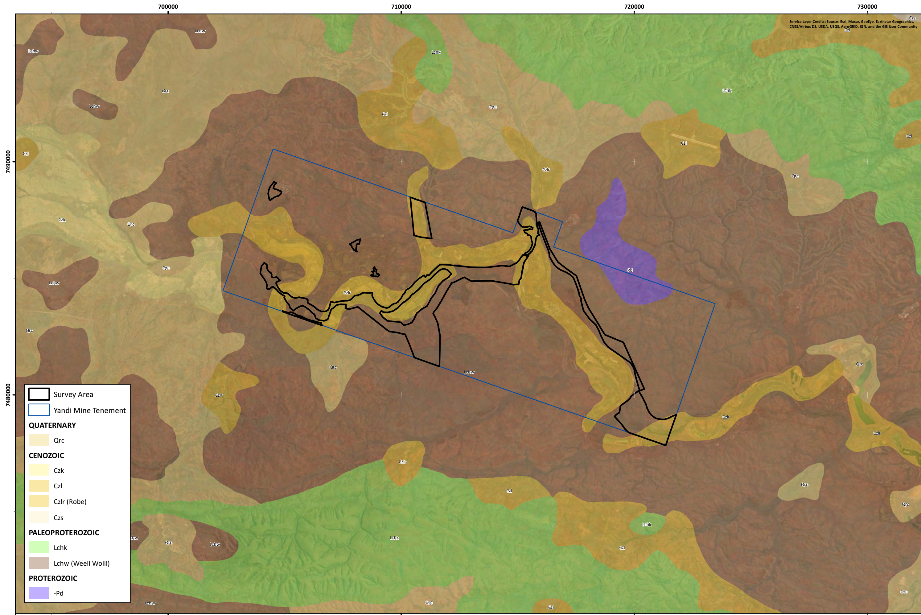
Figure 3: Geological units of the survey area
