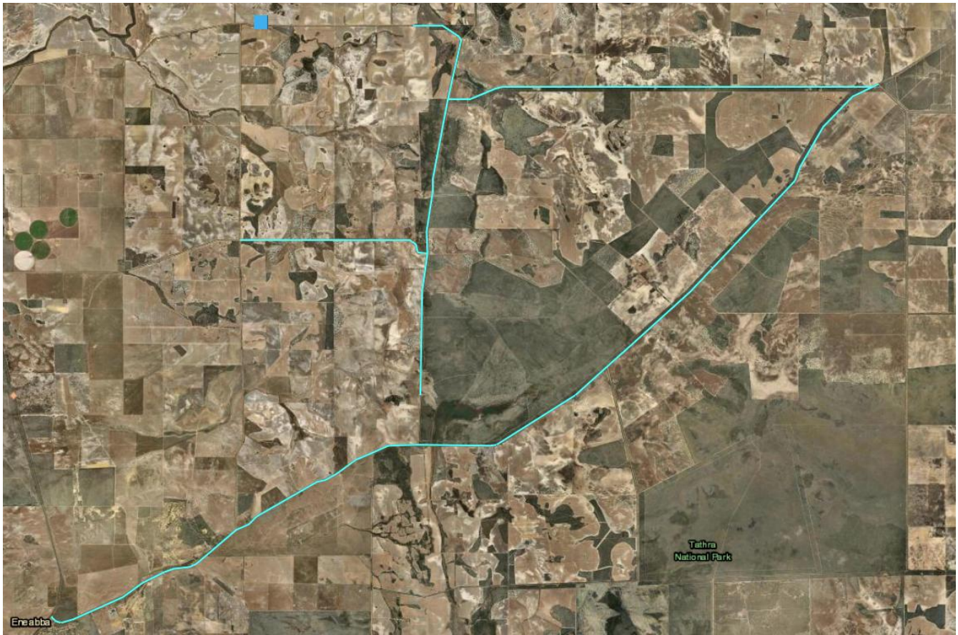
Figure 3-10: Reported Crashes (2020-2024)
